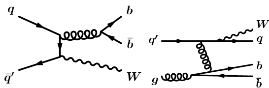
FIG. 1: Feynman diagrams for W + b -jet production.
