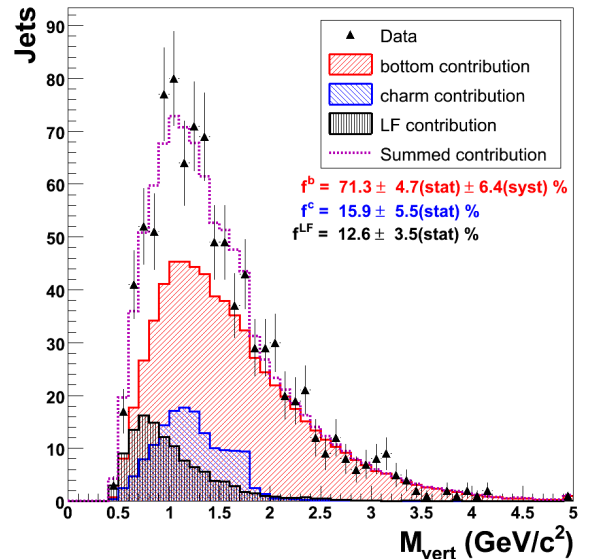
FIG. 3: Maximum likelihood fit of the vertex mass for tagged jets in the selected data sample.
