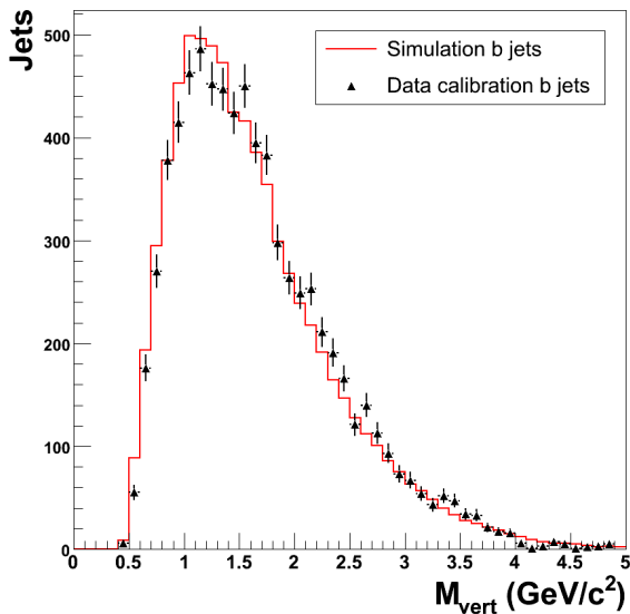
FIG. 2: Comparison of the vertex mass distributions of tagged b jets from dijet simulation sample (histogram) and dijet data sample (triangles).
