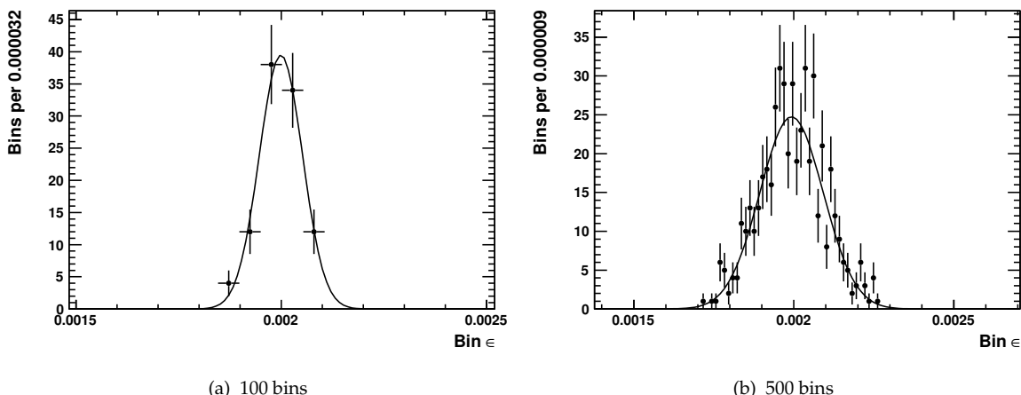
Figure 3: The bin efficiency distributions distributions for 100 bins (a) and 500 bins (b).
