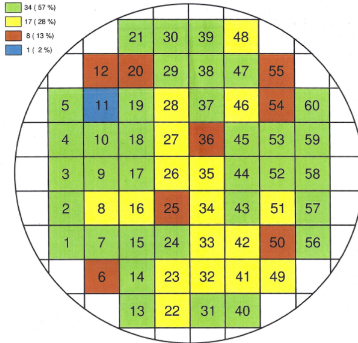
wafer map for wafer VMB8WDH (60 chips)
