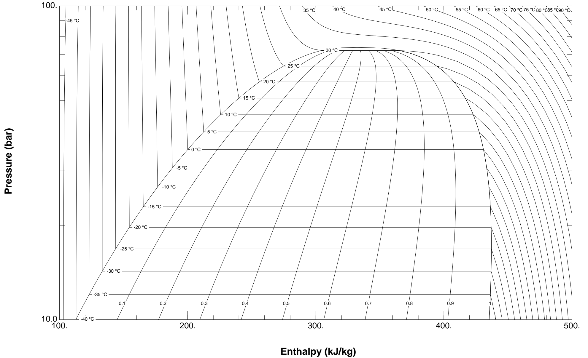
14: Pressure vs. Enthalpy plot: carbon dioxide
