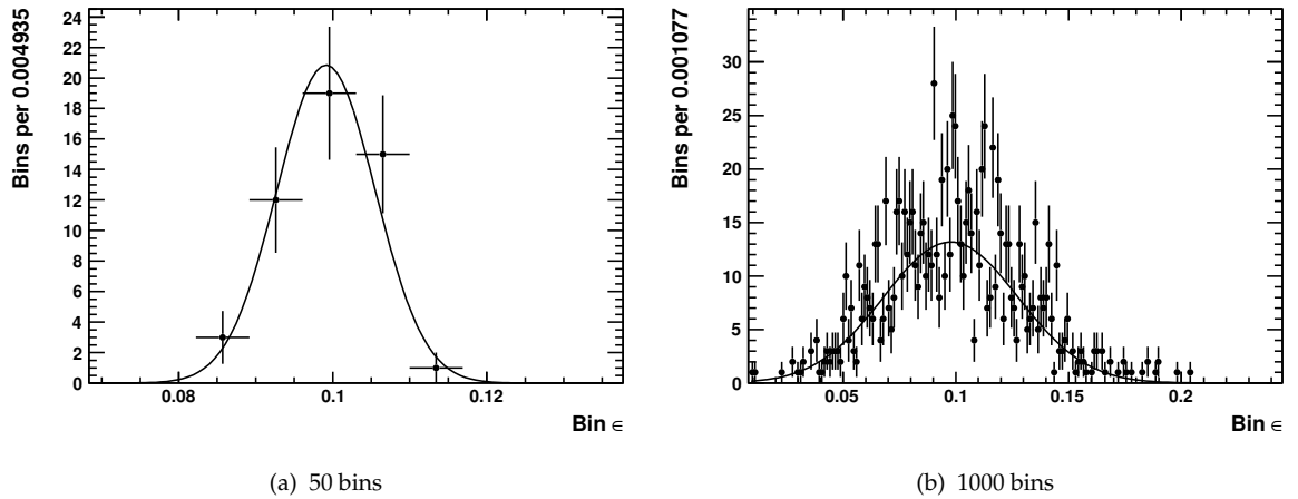
(a) 50 bins (b) 1000 bins Figure 1: The bin binomial efficiency distributions distributions for 50 bins (a) and 1000 bins (b).
